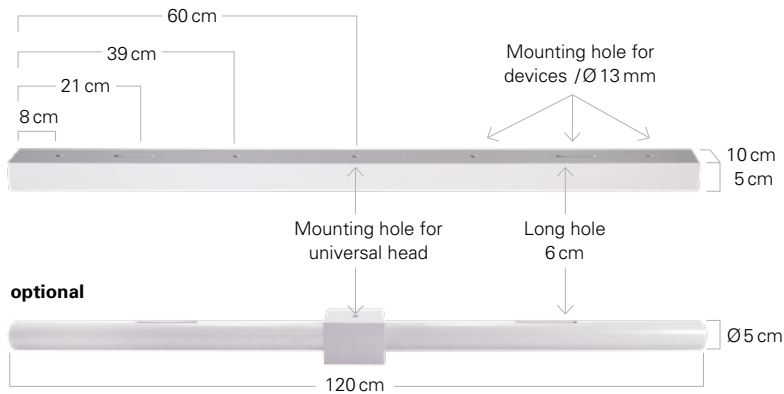
Universal T-Bar (square-shaped or round)
